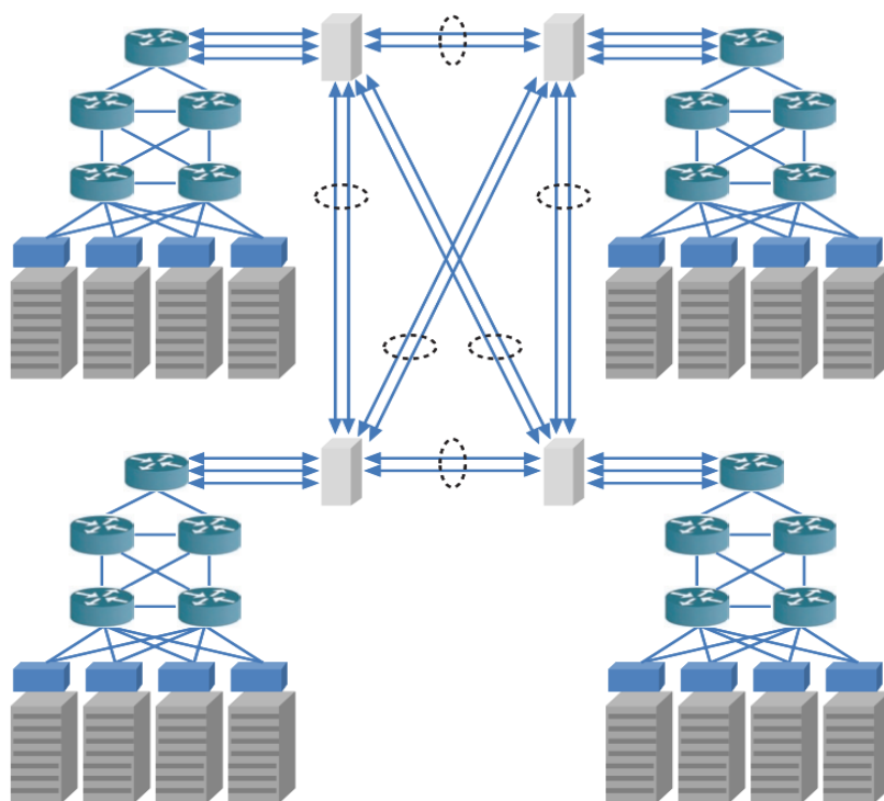
FIGURE 1: Prototypical Meshed Optical Data Center Interconnect Network
